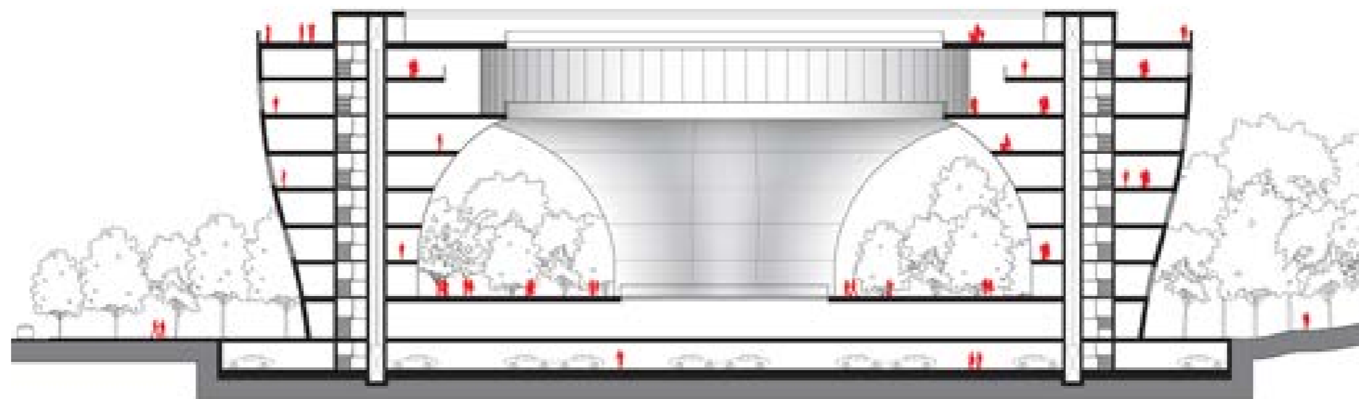
Section B-B
