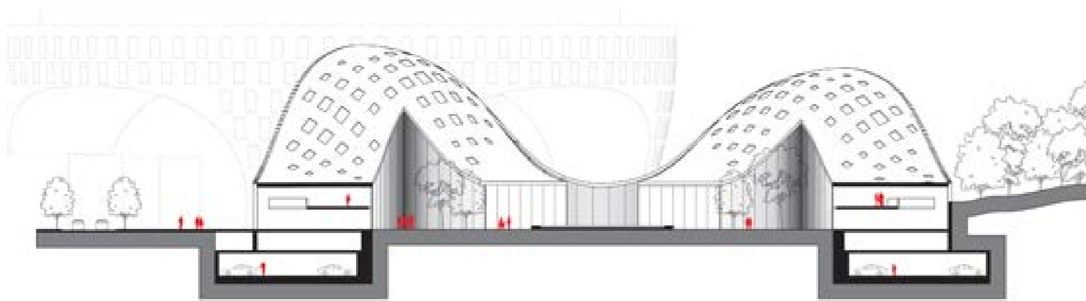
Section B-B
