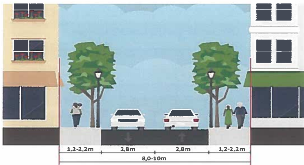
RRUGË LOKALE (F), 8-10m
