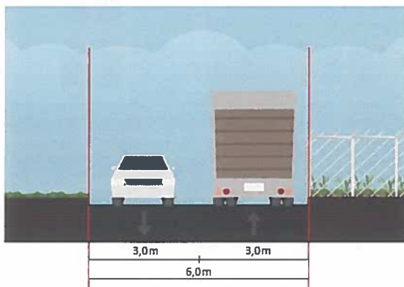
RRUGË LOKALE (F), 5-6m
